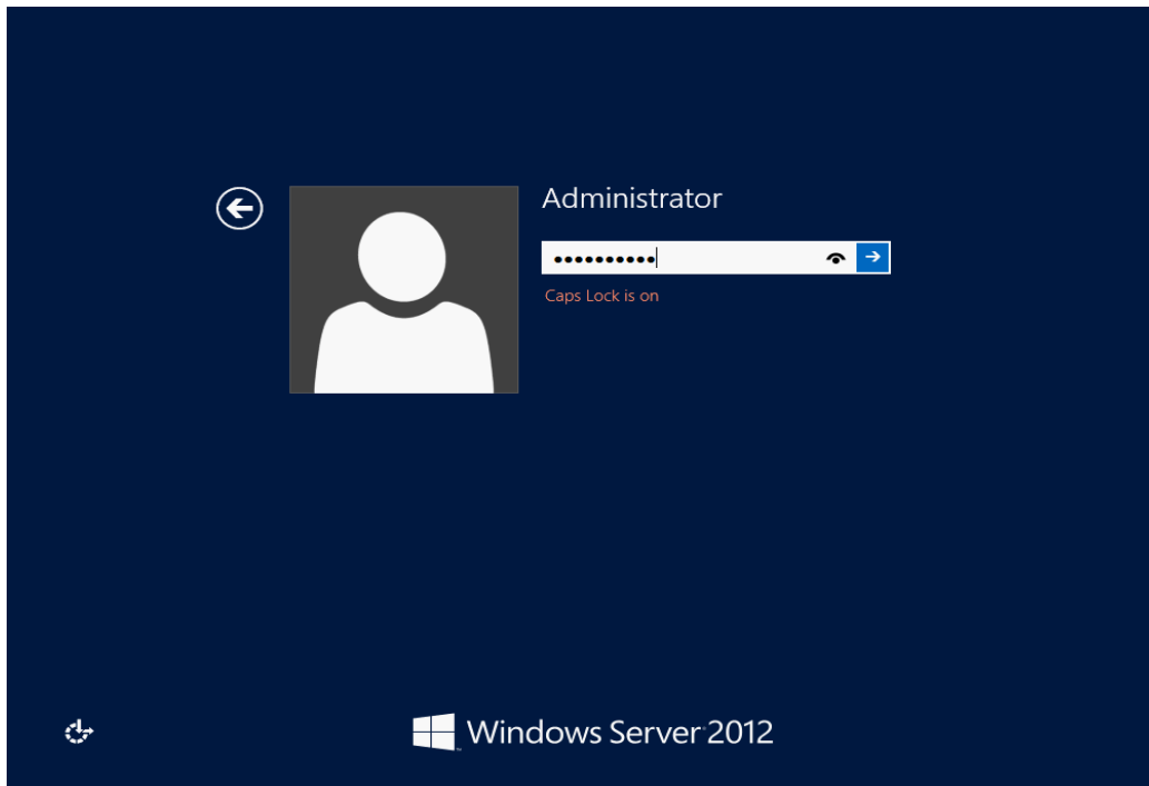
Figure 5-7: Logon Screen
