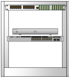
Figure D6: MDF Rack in Small or Full Admin Charter School Site
