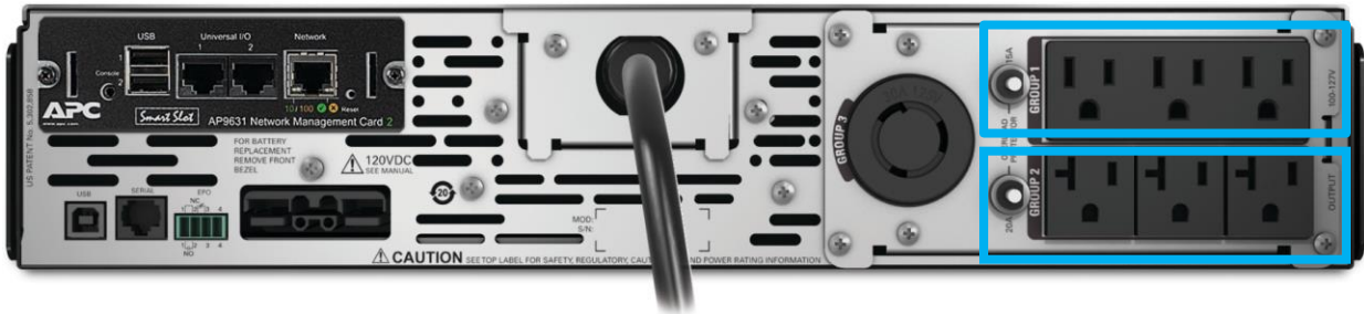
Figure 4-37 - UPS Connections
