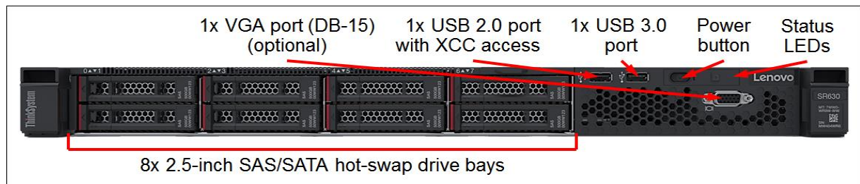
Figure 5-1: Front View of Server
